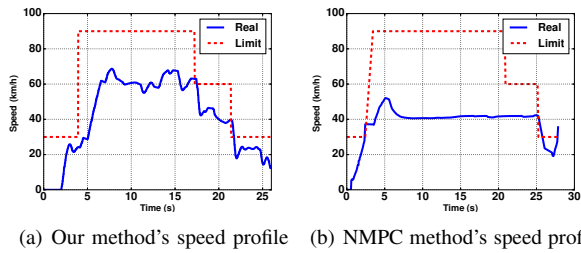
Fig. 5. Speed profiles of the algorithms. Our algorithm reaches higher legal speeds on average, compared to the NMPC implementation.
